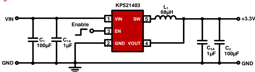
图 32 V_{IN} = 12V , V_{OUT} = 3.3V , I_{OUT} = 1A
